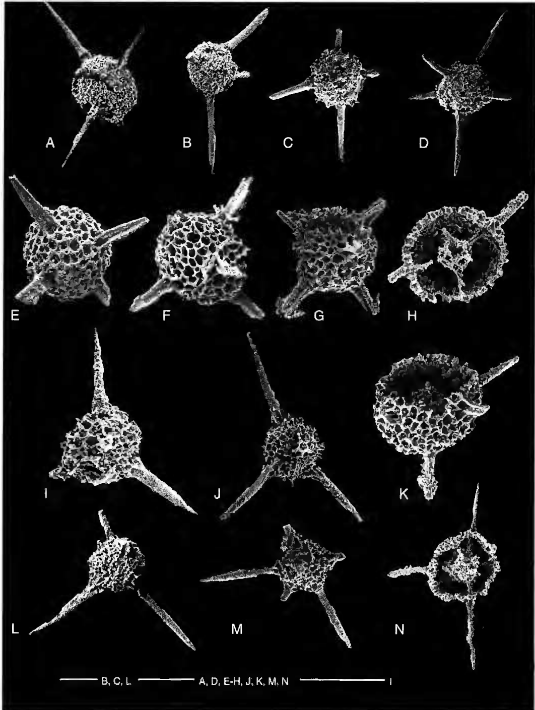
FIG. 10. — A-D, Entactinosphaera (?) sashidai Kamata n. sp., A, holotype, DEUY-YK3483, B, paratype, DEUY-YK3490; C, paratype, DEUY-YK3508; D, paratype, DEUY-YK3434; E-H, Thaisphaera (?) igoi Kamata n. sp.; E, paratype, DEUY-YK3637; F, holotype, DEUY-YK3647; G, paratype, DEUY-YK3655; H, showing internal structure, paratype, DEUY-YK3622; K, paratype, DEUY-YK3591; I, J, L-N, Entactinosphaera chiakensis Sashida & Igo, I, DEUY-YK3492; J, DEUY-YK3520, L, DEUY-YK3421; M, DEUY-YK3433; N, showing inner shell, DEUY-YK3485. Scale bars: 100 \mu m.
